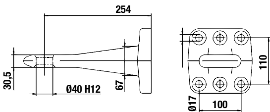
T440 50 15 - VISSERIE INCLUSE
