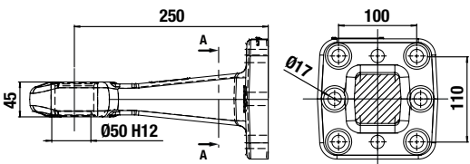
T450 50 15 - VISSERIE INCLUSE
