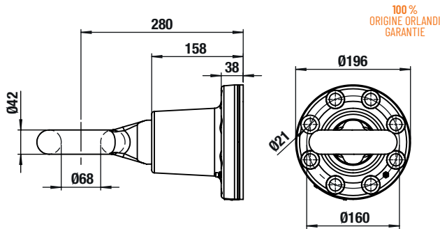
T468 50 35 (VISSERIE INCLUSE)
