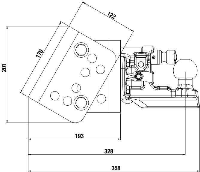
SUPPORT INCLINABLE
